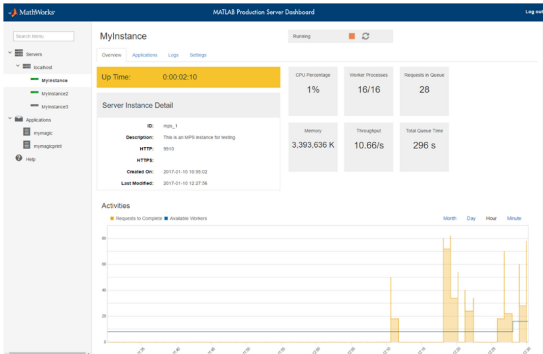
Figure 24. Monitoring metrics using the MATLAB Production Server web dashboard.
