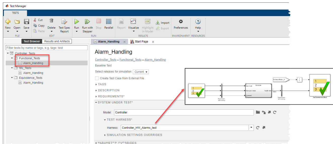
Figure 2. Simulink Test implementing an alarm handling test case by calling a test harness model to exercise a design model. In the harness, the Test Sequence block provides the test vector inputs while a Test Assessment block checks the outputs.
