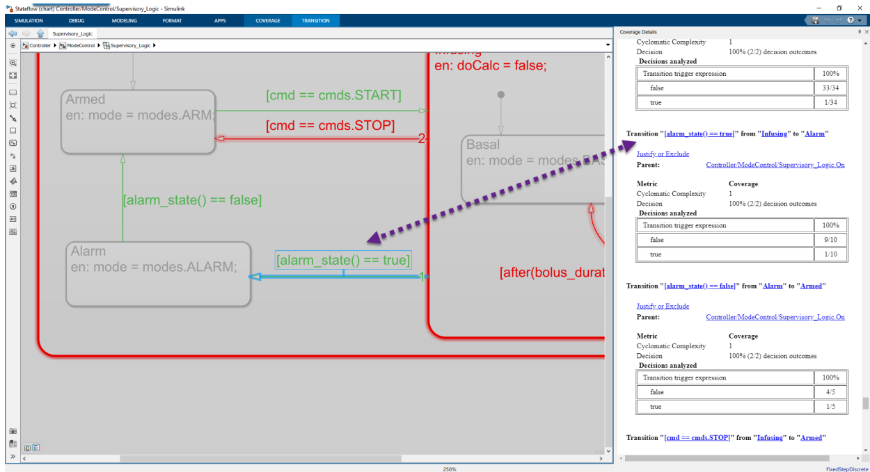
Figure 3. Model highlighted with coverage results. The behavior (Stateflow chart) on the left shows that the alarm was detected, and the HTML report on the right provides a summary artifact. Embedded hyperlinks provide traceability to the model under test.
