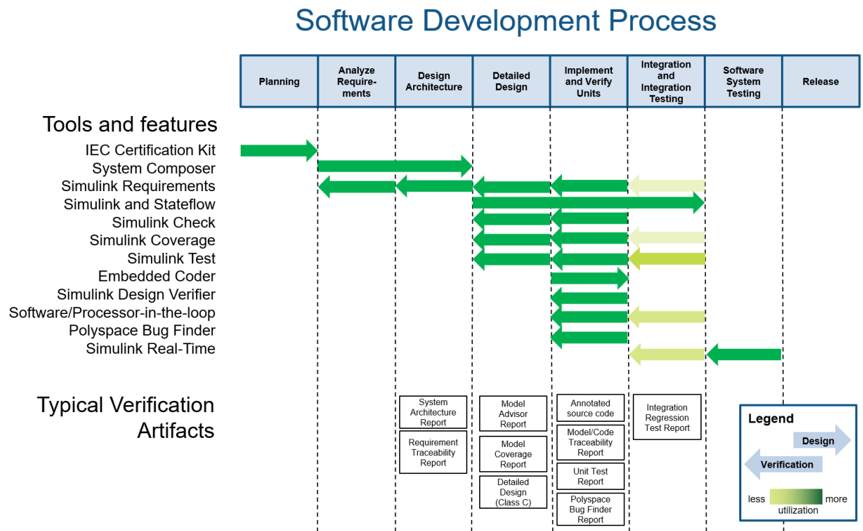
Figure 4. Applicability of Model-Based Design tools for IEC 62304-compliant software development.
